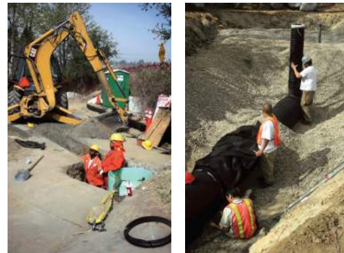
Installing catch basin in Oros Street and drain pipe in park
